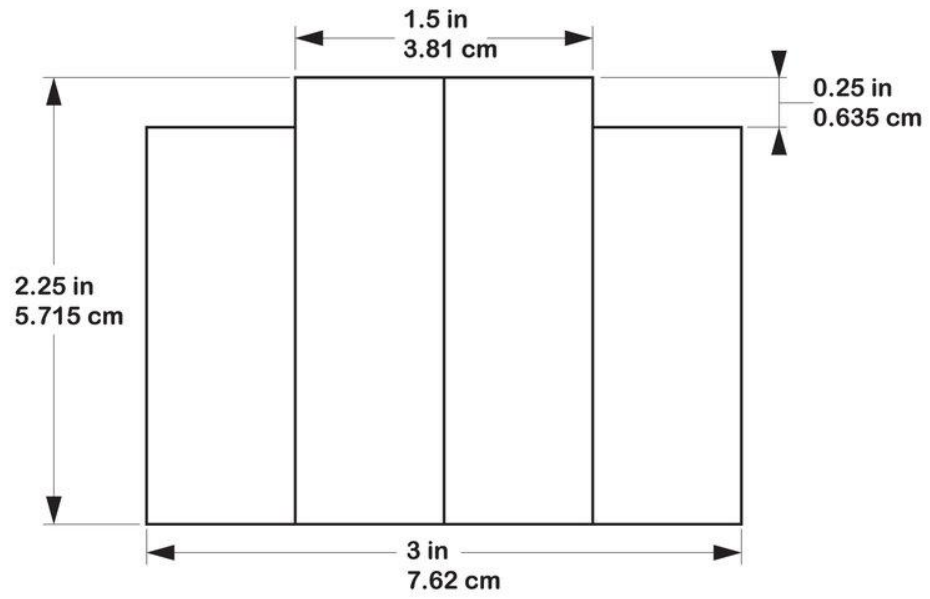
Nerdy Derby Track Cross Section
